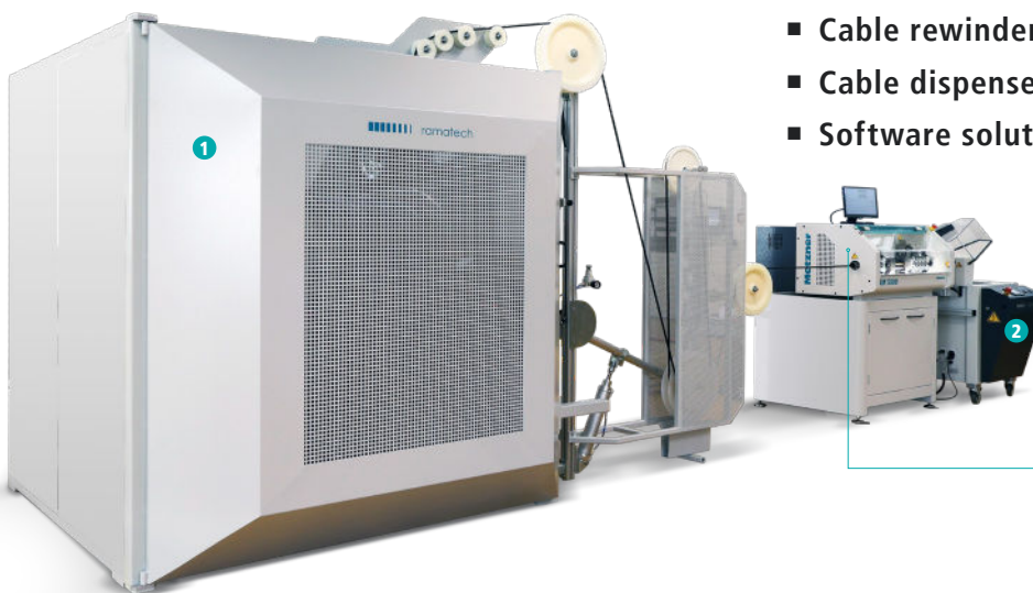
AM 5800 expanded into a production line with 1) electric pay-off for large cable drums and 2) ring coiler
